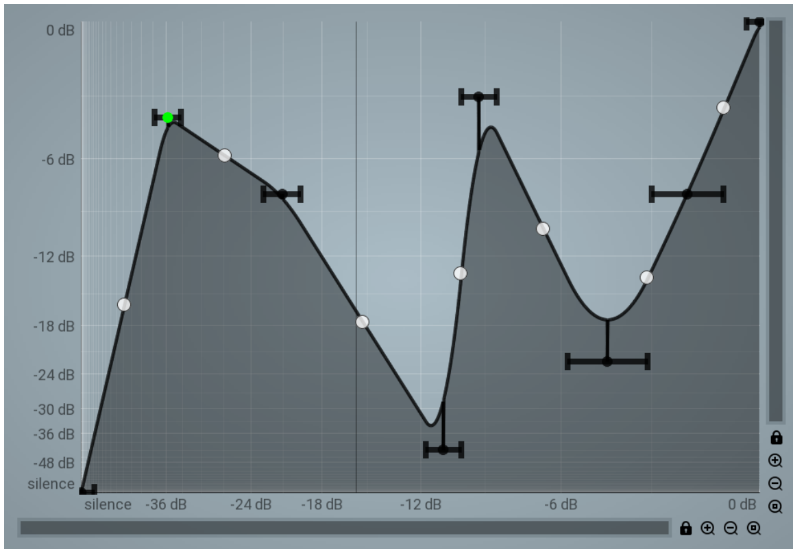
Signal graph
