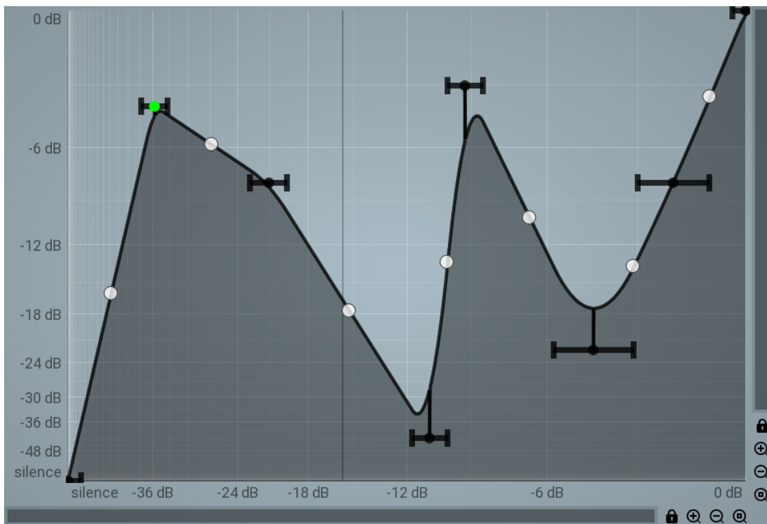
Graph editor
